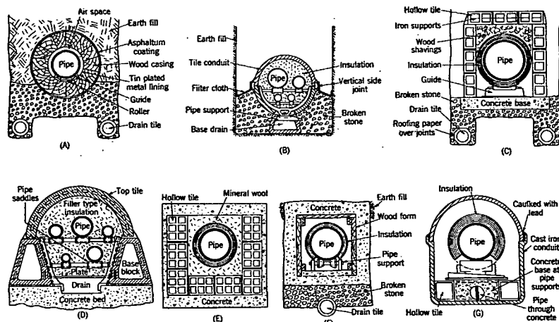
FIG. 1. CONSTRUCTION DETAILS OF CONDUITS COMMONLY USED
