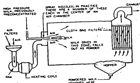
FIG. 15. SPRAY DRYER OF THE PRESSURE-SPRAY ROTARY TYPE 4
