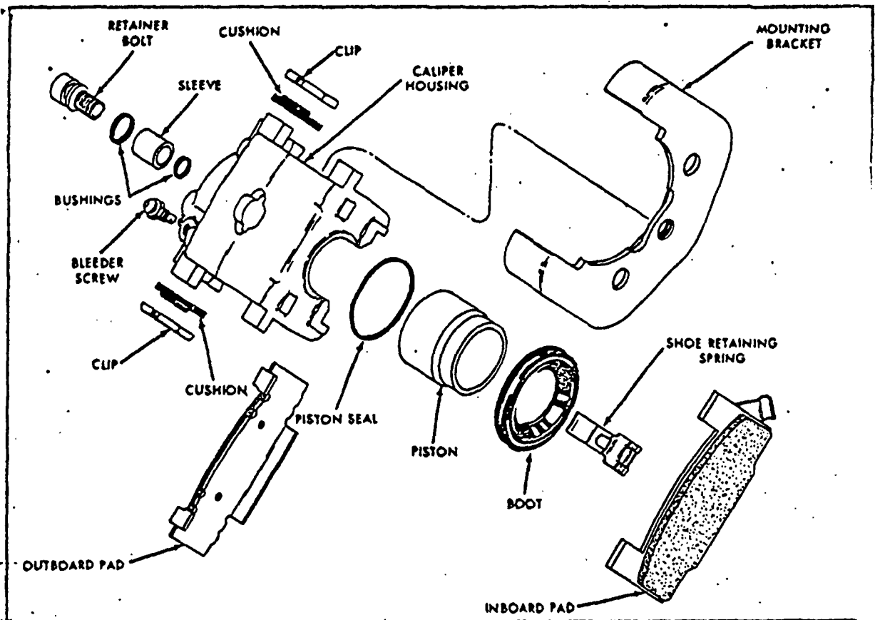
1978-76 CHEVETTE SINGLE PISTON DISC BRAKE
