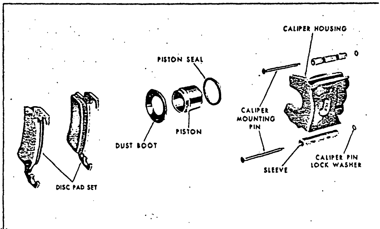
1977-71 VEGA TYPE SINGLE PISTON DISC BRAKE
