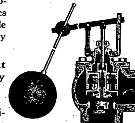
No. 7 Single Seated Float Valve
