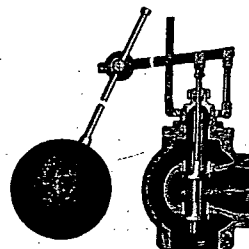
No. 6 Balanced Float Valve
