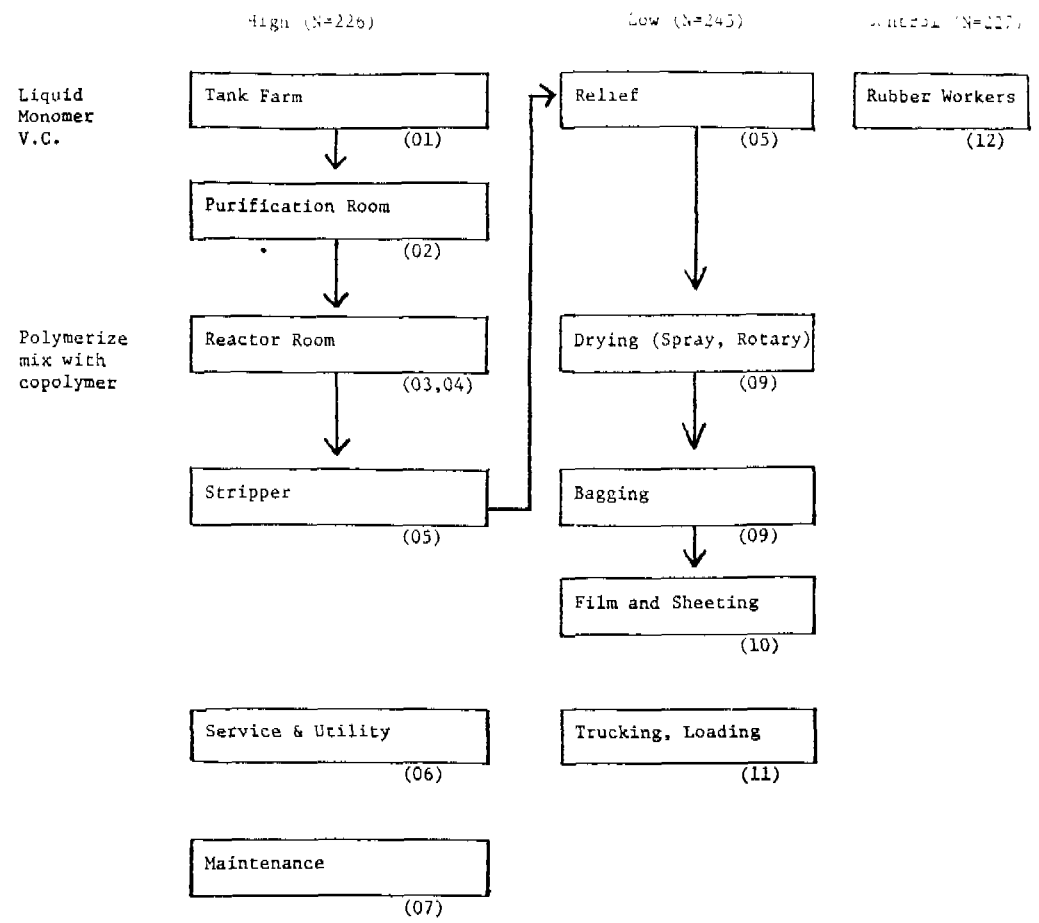
( ) Denotes O.T. from Table I. Figure 1 - Schematic flow diagram of vinyl chloride polymerization.
