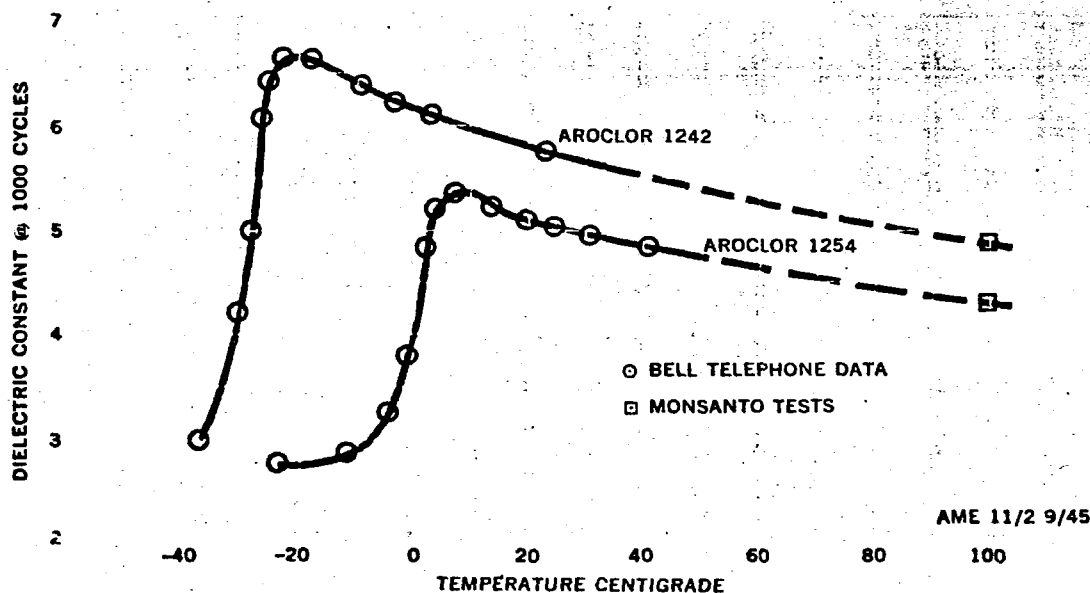
DIELECTRIC CONSTANT VS. TEMPERATURE AROCLOR 1242 & AROCLOR 1254
