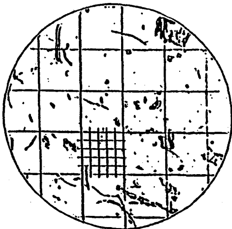
FIGURE 1. PHOTOMICROGRAPH OF DUST FROM AN ASBESTOS FABRICATING PLANT. MAGNIFICATION 800 DIAMETERS
