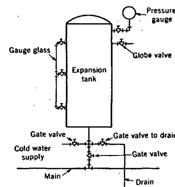
FIG. 10. A CLOSED EXPANSION TANK
