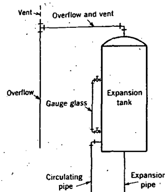
FIG. 9. AN OPEN EXPANSION TANK
