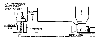
Fig. 13...Control of Preheat Coil From Outdoor Air
