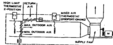
Fig. 12...All-Season Ventilation Control With Fixed Minimum Outdoor Air Plus Additional Outdoor Air When Practicable
