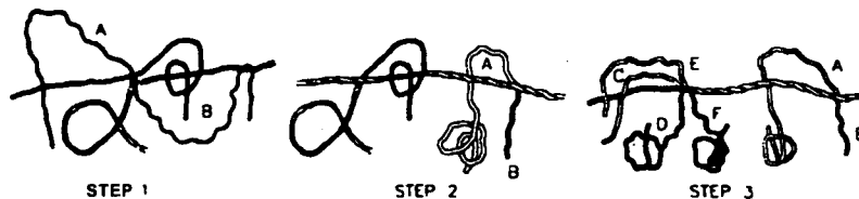
Figure 15-3. Making a short splice
