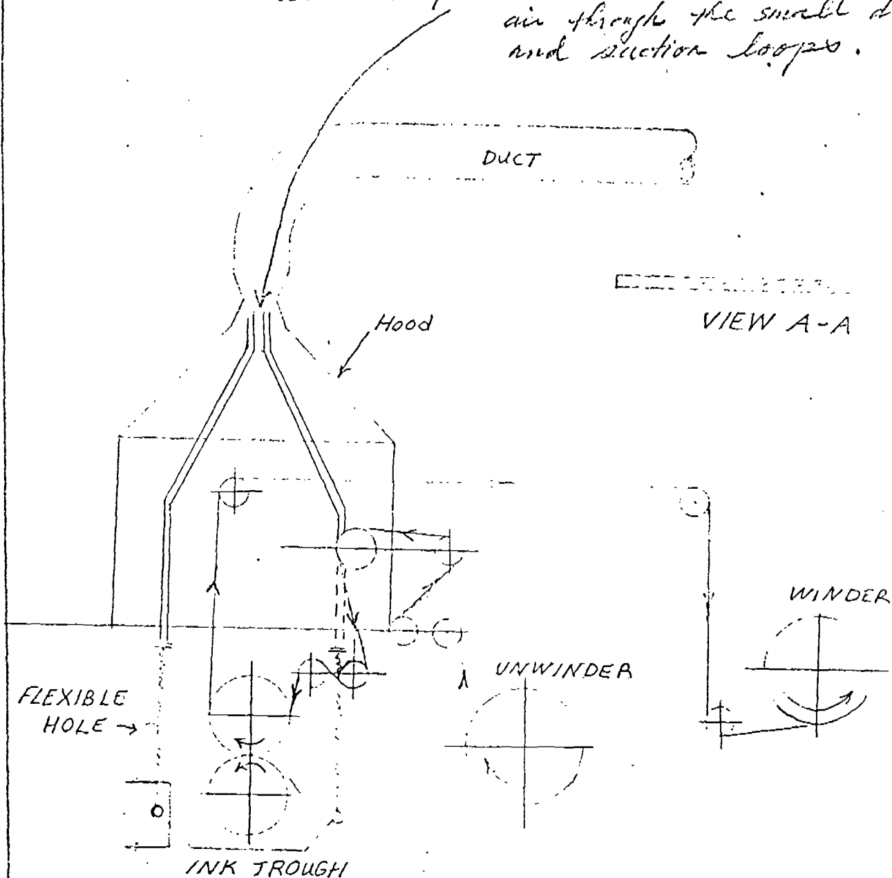
Drawing No. 2 schematic drawing - solvent control for SINGLE COLOR PRINT MACHINE
