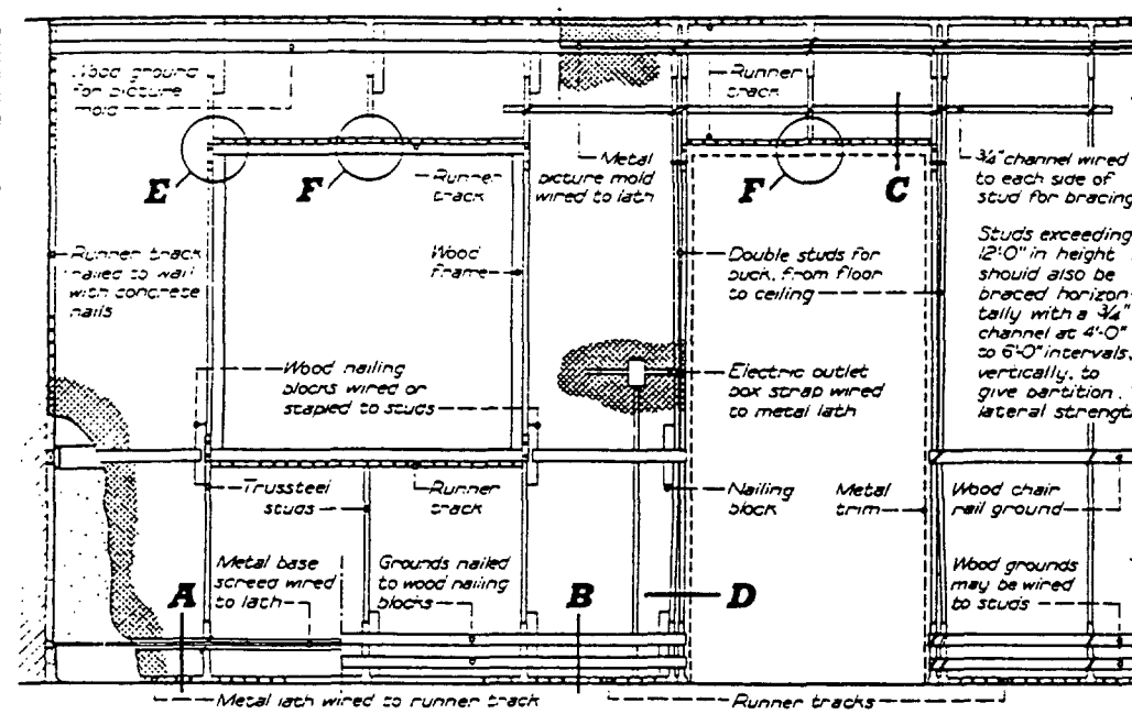
Elevation of Trusstee Stud Partition.
