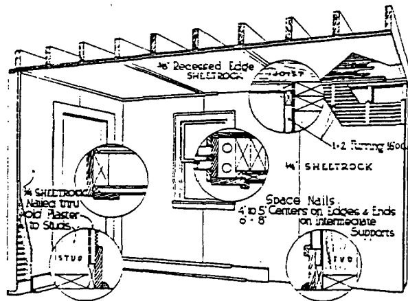
APPLICATION OF SHEETROCK OVER OLD PLASTER
