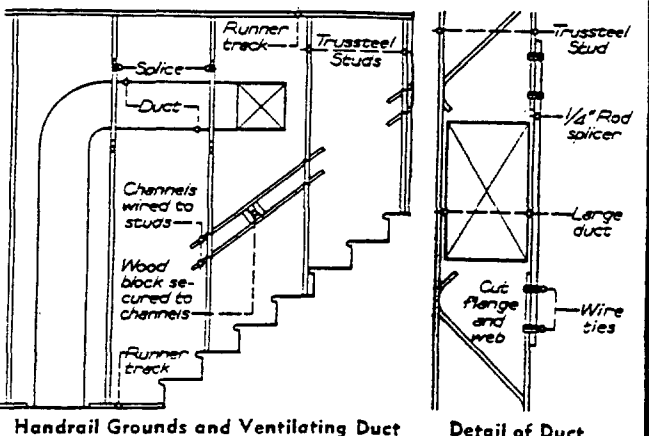
Wood Frame for Window or Other Openings
