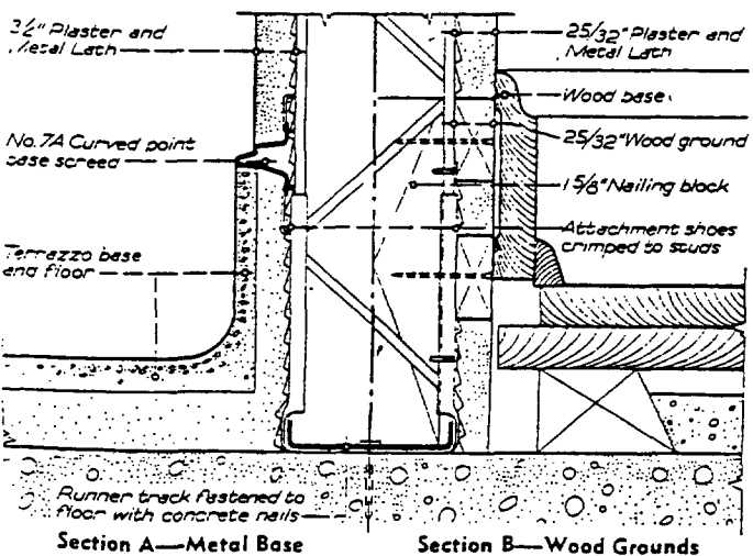
Section A—Metal Base
