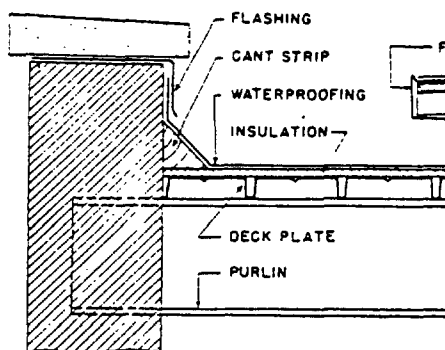
DETAIL AT PARAPET
