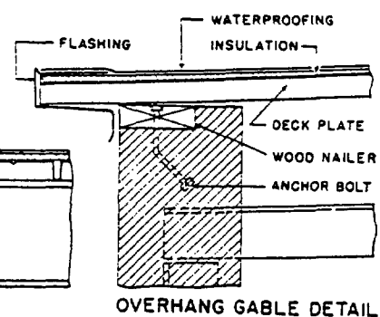
OVERHANG GABLE DETAIL
