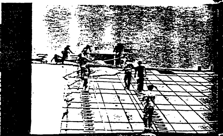
Pyrofill, plastic gypsum material, is poured over fabric and permanent form.
