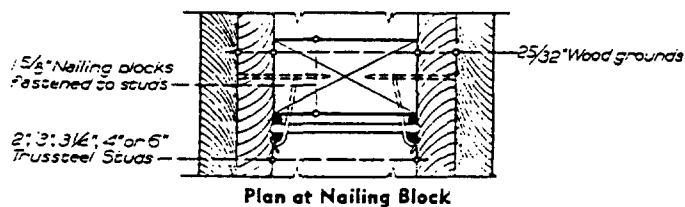
Plan at Nailing Block
