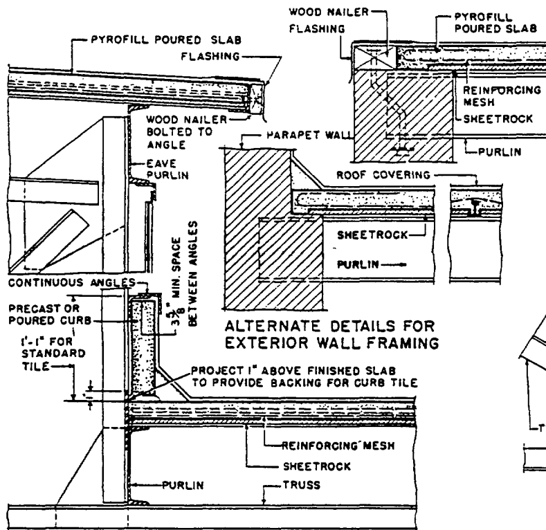
CURB AND EAVE CONSTRUCTION FOR MONITOR
