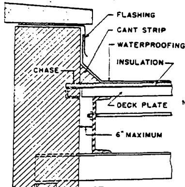
DETAIL AT PARAPET
