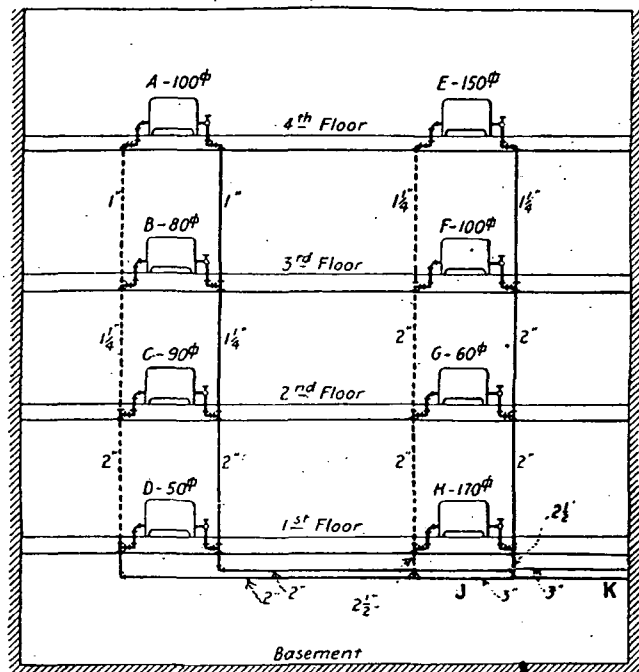
FIG. 38. LAYOUT FOR SIZING HOT WATER MAINS
