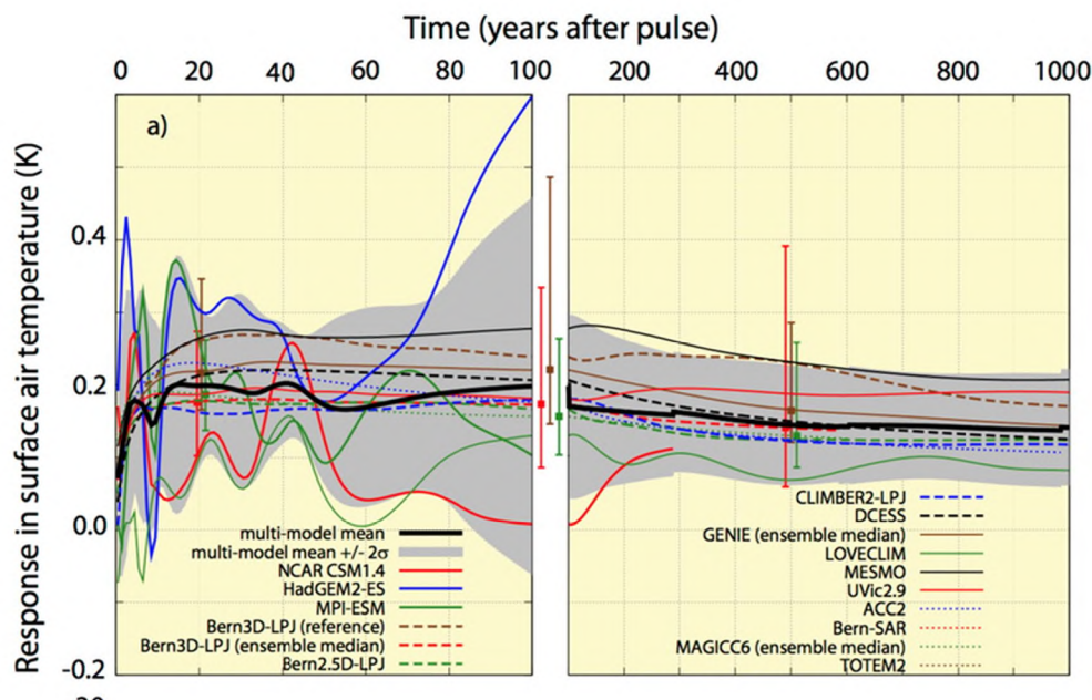
FIGURE 3-7 Response of global mean temperature to a 100 GtC pulse emission of CO 2 . NOTES: The data are from the same experiments shown in Figure 3-4 (above), with temperature change expressed relative to a stable baseline CO 2 concentration of 389 ppm. Participating full-complexity Earth system models (solid curves) have a high degree of variability. The Earth system models of intermediate complexity and simple climate models are shown with dashed and dotted lines, respectively. SOURCE: Joos et al. (2013, Figure 2a).
