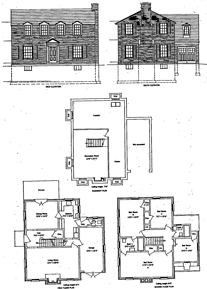
FIG. 1. ELEVATIONS AND FLOOR PLANS OF RESIDENCE
