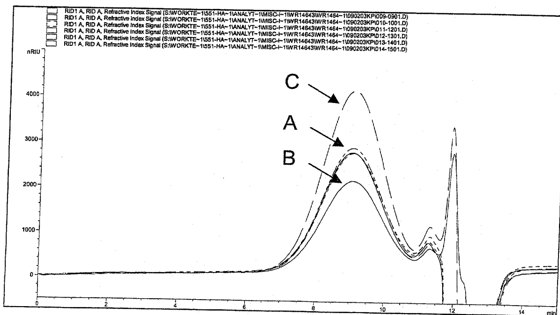
Figure 2: LC chromatograms of four Day 5, pH 4.0 replicate samples (A), 7500 mg/L (B), and 15000 mg/L (C) calibration standards of [REDACTED]
