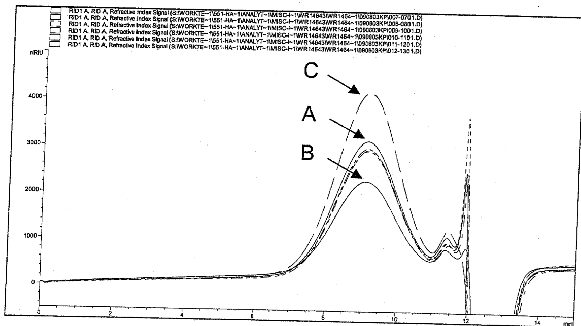
Figure 4: LC chromatograms of four Day 5, pH 9.0 replicate samples (A), 7500 mg/L (B), and 15000 mg/L (C) calibration standards of [REDACTED]
