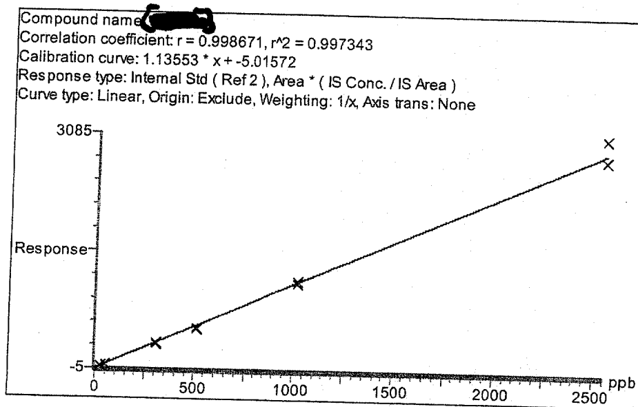
Figure 6: Representative calibration curve for [REDACTED]
