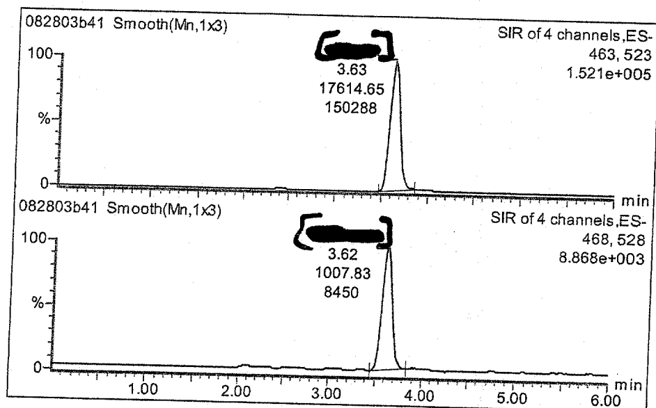
Figure 8: Representative chromatograms for Day 0, pH 4.0 hydrolytic stability sample and 520 µg/L [redacted] internal standard.
