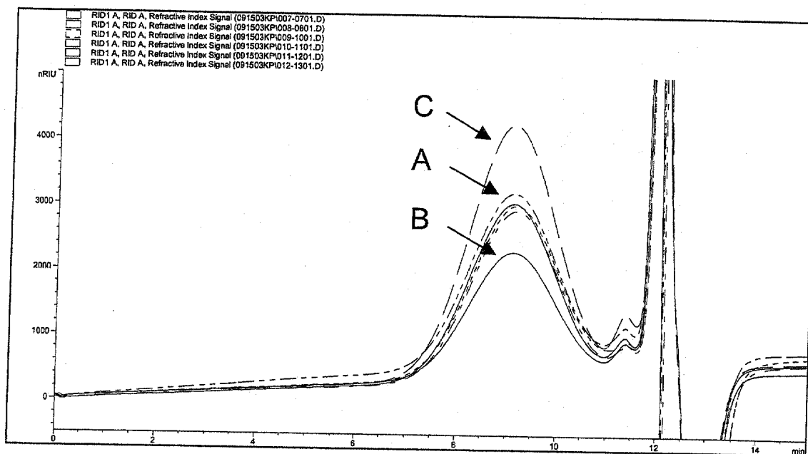
Figure 1: LC chromatograms of four Day 5, pH 1.2 replicate samples (A), 7500 mg/L (B), and 15000 mg/L (C) calibration standards of [REDACTED]
