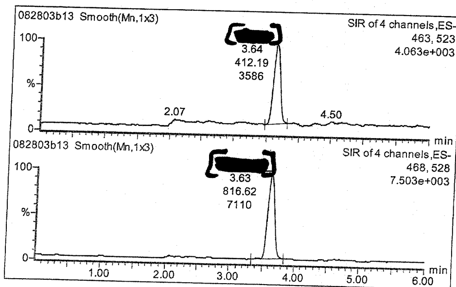
Figure 7: Representative chromatograms of 25.5 µg/L [REDACTED] calibration standard and 520 µg/L [REDACTED] internal standard.
