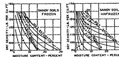
Fig. 3.... Determining Thermal Conductivity of Soils from Density and Moisture Content
