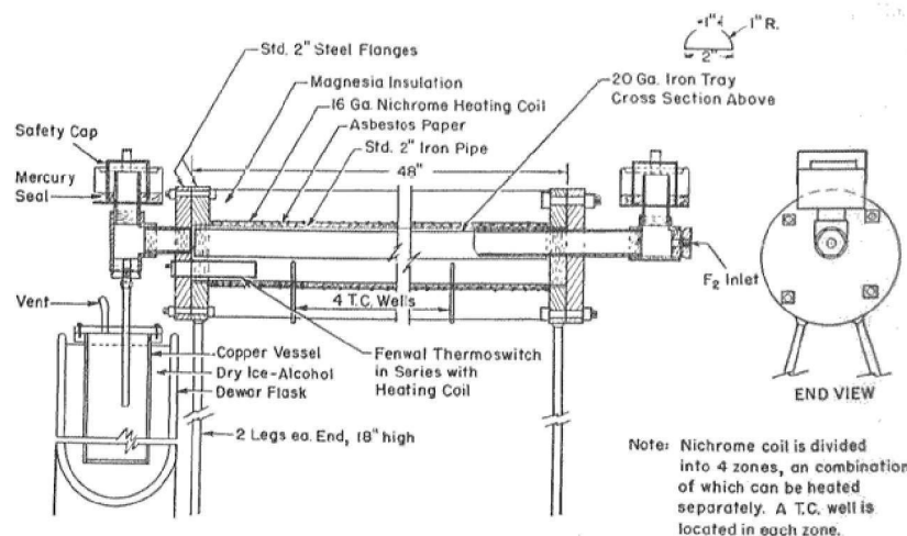
FIG. 2.—Apparatus used in the mercury catalyzed reaction between fluorine and carbon.
