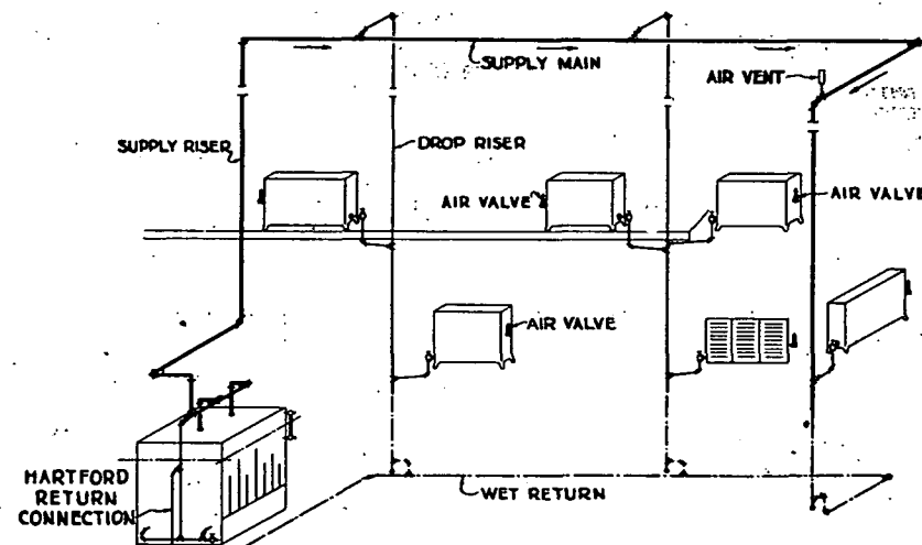
FIG. 2. TYPICAL GRAVITY ONE-PIPE DOWN-FEED STEAM SYSTEM
