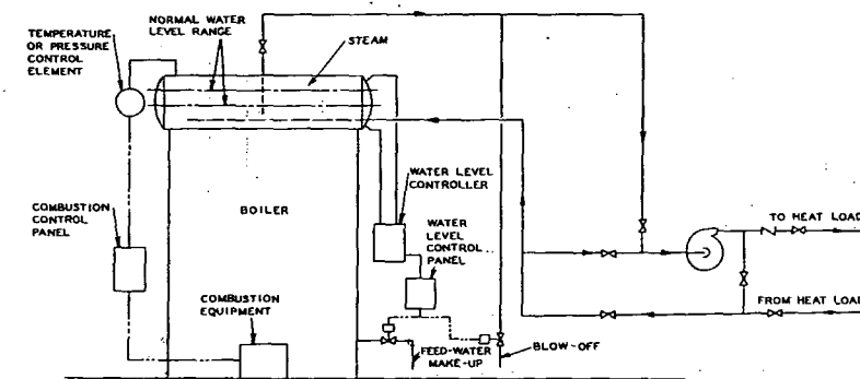
Fig. 4 .... Schematic Arrangement of Combustion and Feed-Water Controls
