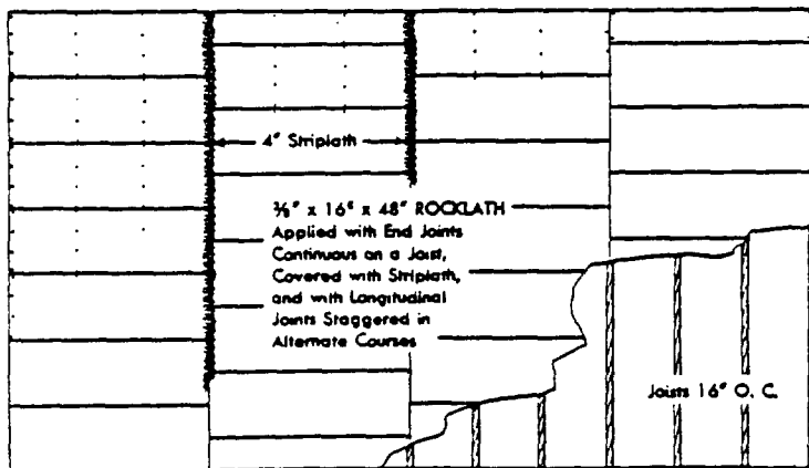
FIG. 2. Alternate Ceiling Application (Canadian system)
