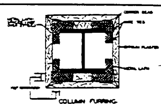
COLUMN FURRING
