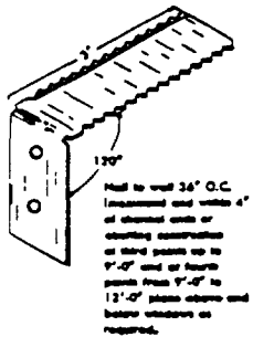
USG—ADJUSTABLE WALL FURRING BRACKET
