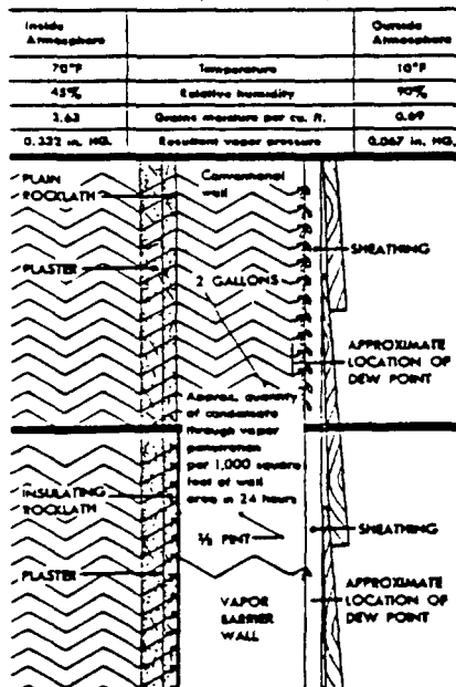
Illustration of Importance of Vapor Barrier
