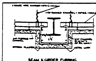
BEAM & GIRDER FURRING
