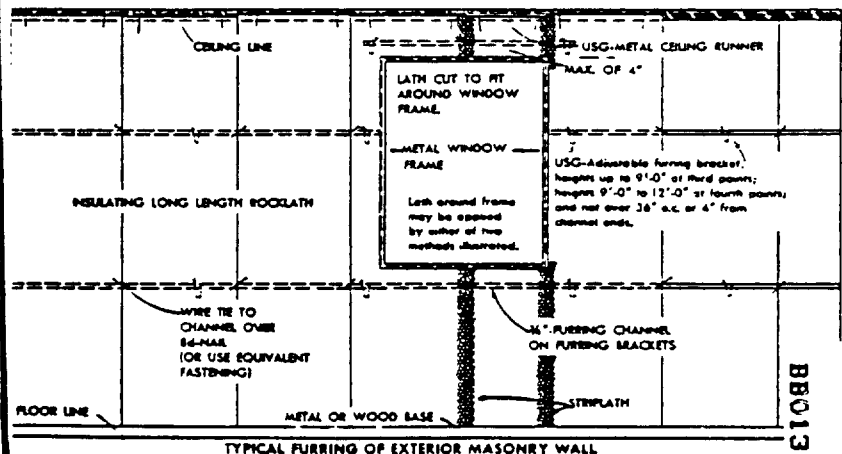
TYPICAL FURRING OF EXTERIOR MASONRY WALL
