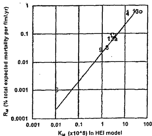
Fig. 10. Comparison of alternative measures of mesothelioma mortality.
