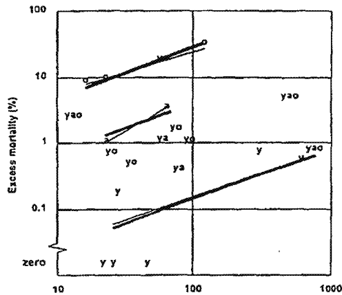
Fig. 6. Excess mortality from pleural mesothelioma against cumulative exposure, showing fibre type. Regression lines fitted to pure fibre cohort. Bold lines indicate fits with slope constrained to be common across fibre types, narrow lines are unconstrained fits.
