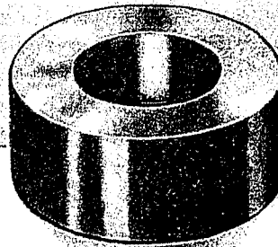
STYLE #776-S —Endless or split molded rings of the same construction as Style 772-S, impregnated throughout with graphite for extra lubrication value. Recommended for the same services as Style 776, but where extra-free motion is desired.
