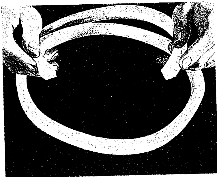
Braided "Teflon" fiber packing, impregnated with dispersion of "Teflon" resin, has that cool, white look. Removal of heat-generating particles means higher speed uses; added resin improves seal, reduces leakage.
