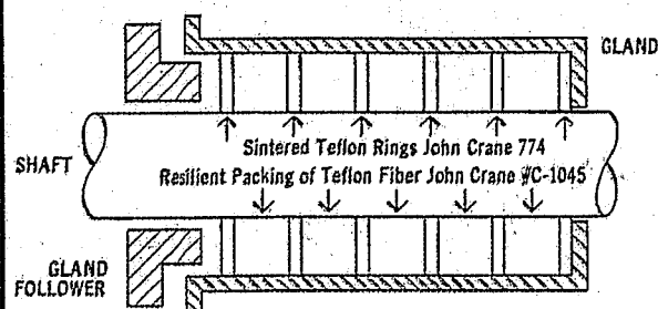
Fig. 1—Combination Packing with Labyrinth Seal
