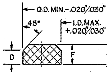
MALE ADAPTER
