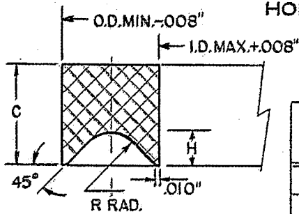
FEMALE ADAPTER
