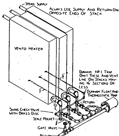
Typical connections using Thermostatic and Float Trap on a Vento Heater
