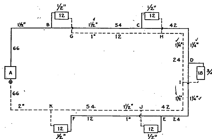
FIG. 3. A FORCED CIRCULATION REVERSED RETURN SYSTEM a
