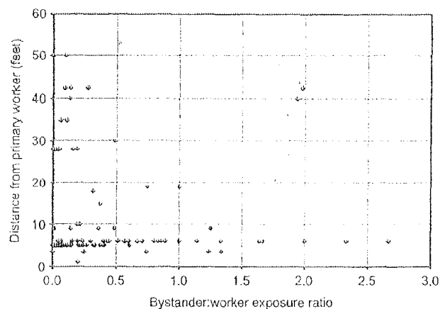
Figure 4. X-Y scatter plot for published data, bystander:worker ratios of airborne asbestos concentrations at distance from a source
