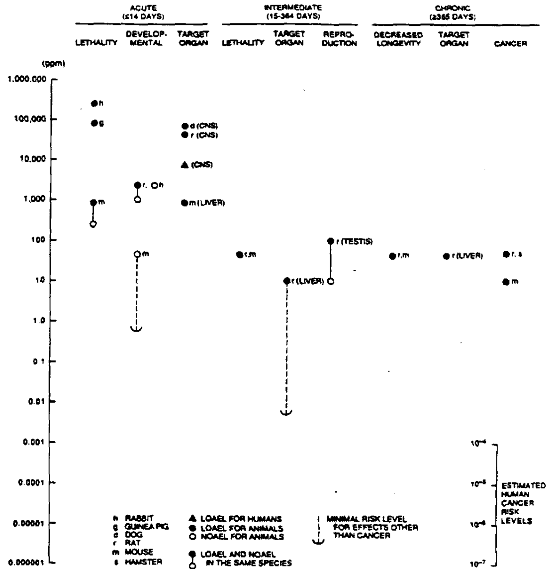
Fig. 2.3. Levels of significant exposure for vinyl chloride—inhalation.
