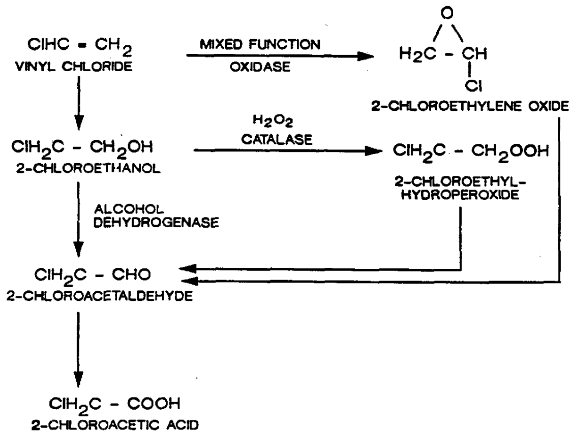
Fig. 4.1. Proposed metabolic pathways for vinyl chloride.
