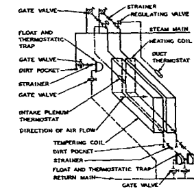
Fig. 58.... Typical Connections to Finned-Tube Blast Heating Coils Arranged for Series Flow of Air
