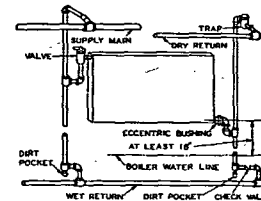
Fig. 55.... Two-Pipe Connections to Radiator Hung on Wall
