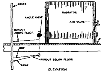
Fig. 53.... One-Pipe Radiator Connections
