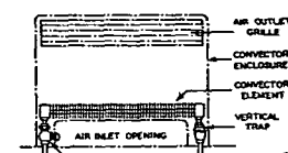
Fig. 56.... Typical Convactor Connections
