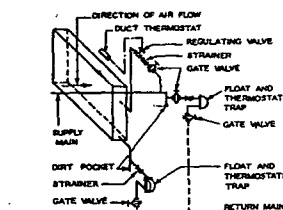
Fig. 60.... Typical Connections to Finned-Tube Blast Heating Coils of the Steam Distributing or Nonfreeze Type
