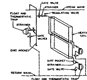
Fig. 59.... Typical Connections to Finned-Tube Blast Heating Coils Arranged for Parallel Flow of Air
