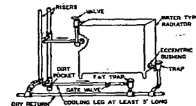
Fig. 54.... Two-Pipe Top and Bottom Opposite End Radiator Connections
