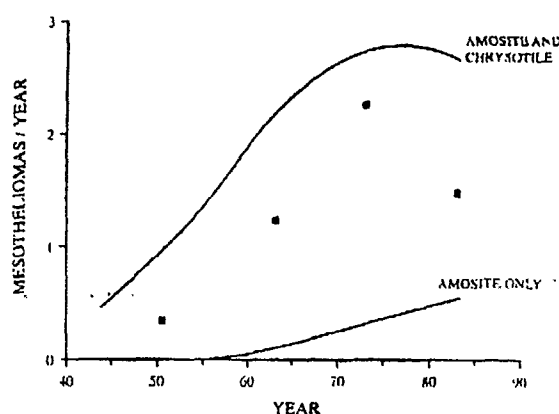
Fig. 1. Estimated and observed cases of mesothelioma/year, 1943-1987 for insulators exposed to amosite alone and amosite/chrysotile. Estimated numbers (smooth curves) are from models of asbestos cancer risk. The solid square represents the number of mesothelioma cases actually observed.
