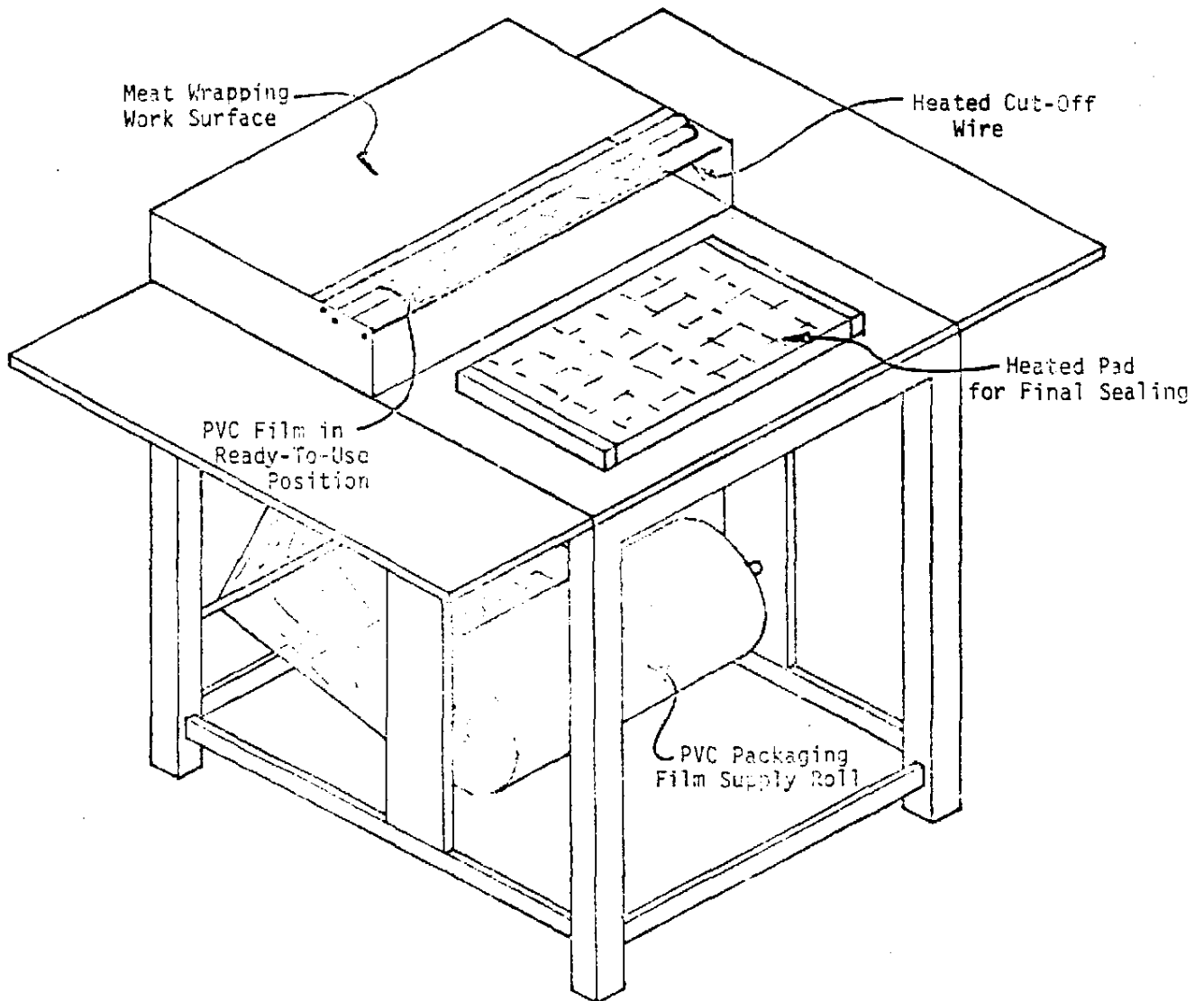
FIGURE 1: Typical Hand-Wrapping Machine
