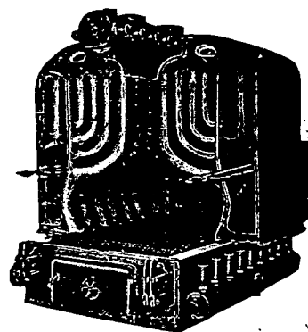
No. 44 Mills Boiler—Interior
