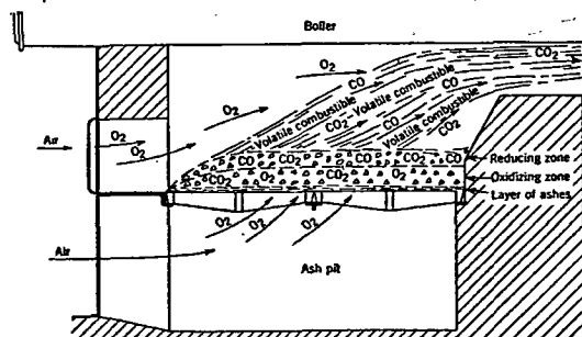
FIG. 1. COMBUSTION OF FUEL IN A HAND-FIRED FURNACE
