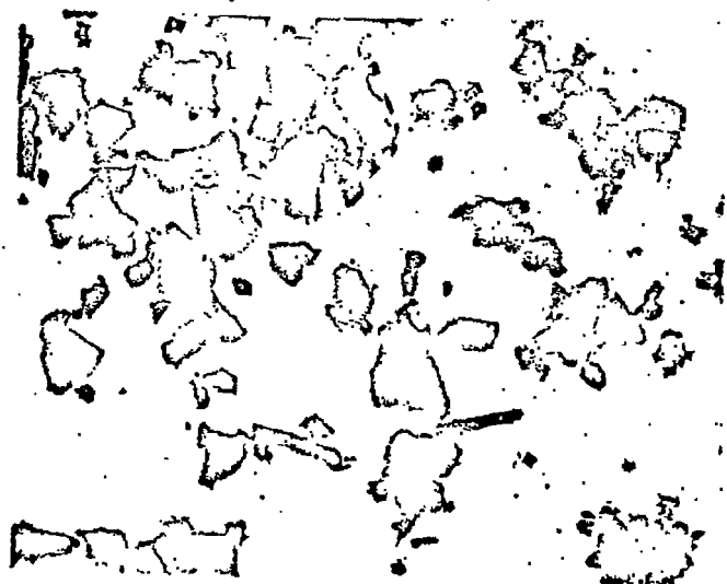
Fig. 4. Specimen I21. Inclusion from Face 2. x 3000. This specimen produced plate-like and compact particles with some lath-like forms.
