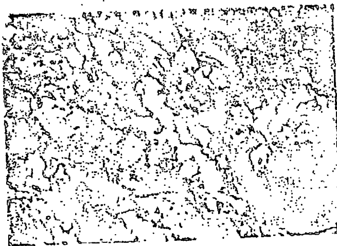
Fig. 22b Photomicrograph, x 24 mag., of thin section I25 under XN.
