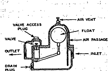
FIG. 21. SINGLE PORT FLOAT TRAP
