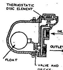
FIG. 25. TYPICAL FLOAT AND THERMOSTATIC TRAP
