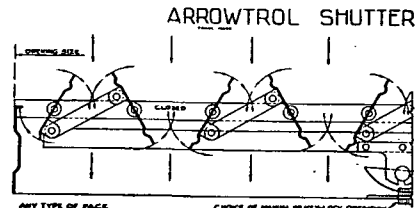
The Arrowtrol, line cut shown above, gives straight throw in connection with volume control
