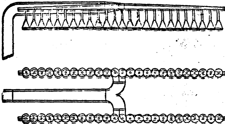
FIGURE 2.—Schematic views of exhaust system applied to Foster winders.
