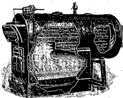
Up-Draft Type
