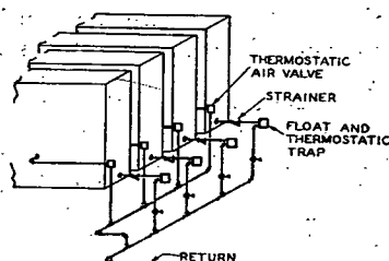
FIG. 40. TYPICAL CONNECTIONS TO CAST IRON BLAST HEATERS MORE THAN 12 SECTIONS LONG
