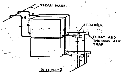
FIG. 39. TYPICAL CONNECTIONS TO CAST IRON BLAST HEATERS LESS THAN 12 SECTIONS LONG
