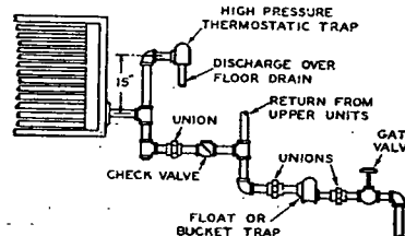
FIG. 42. TYPICAL RETURN CONNECTION FROM FINNED TUBE BLAST HEATERS WITH HIGH PRESSURE STEAM
