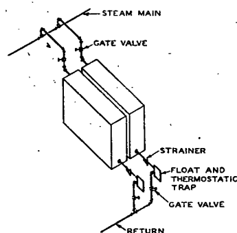
FIG. 41. TYPICAL CONNECTIONS TO FINNED TUBE BLAST HEATERS WITH LOW PRESSURE STEAM
