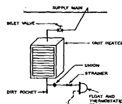
Fig. 62.... Typical Unit Heater Connections for Two-Pipe System
