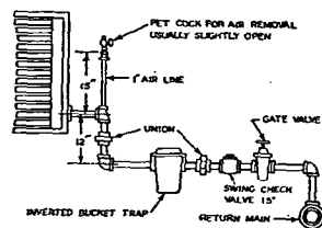
Fig. 61.... Typical Return Connections to Finned-Tube Blast Heaters with High-Pressure Steam
