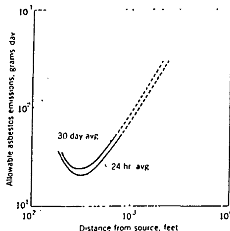
Figure 3. Calculated maximum allowable asbestos emission rate as a function of distance from source (assumed 4 m/sec wind speed, 10m effective stack height, 40% frequency factor for wind direction, and C stability class).
