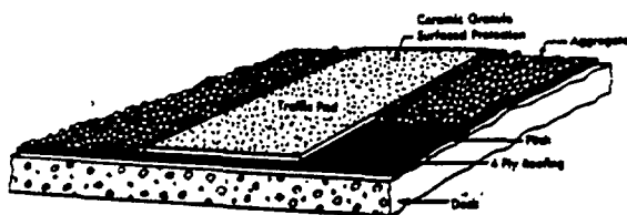
Traffic Pad
