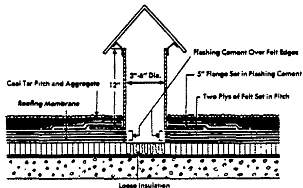
Roof Vent
