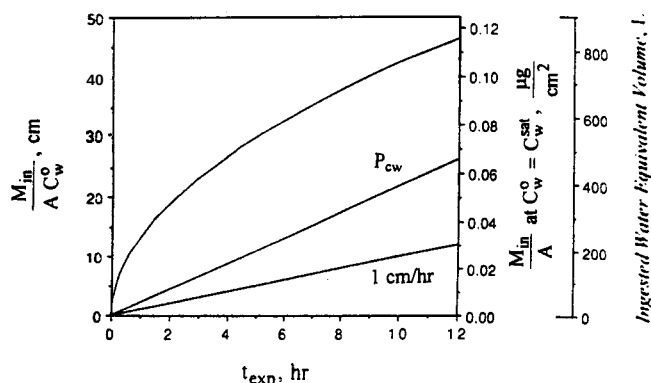
Figure 2. Cumulative mass of dibenz(a,h)anthracene absorbed into the SC as a function of t_{exp} predicted by the B and steady-state expressions.
