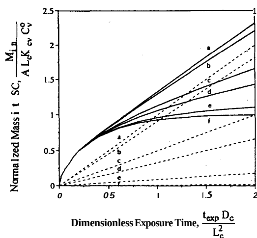
Figure 1 Normalized cumulative mass entering the stratum corneum when the viable epidermis is present plotted as a function of dimensionless t_{exp} and B (a: B \leq 0.01 ; b: B = 0.1 ; c: B = 1 ; d: B = 2 ; e: B = 10 ; f: B \geq 100 ). Solid curves represent the unsteady-state case; dashed lines, the steady-state Eqn. (8).
