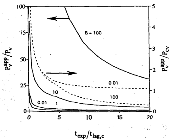
Figure 6. P_v^{app}/P_v and P_v^{app}/P_{cv} as functions of dimensionless t_{exp}/t_{lag,c} .
