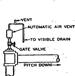
FIG. 12. TYPICAL AUTOMATIC AIR VENT VALVE INSTALLATION
