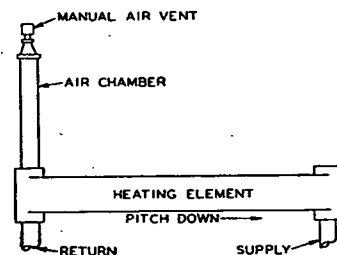
FIG. 13. TYPICAL AIR VENT VALVE INSTALLATION ON HEATING ELEMENT
