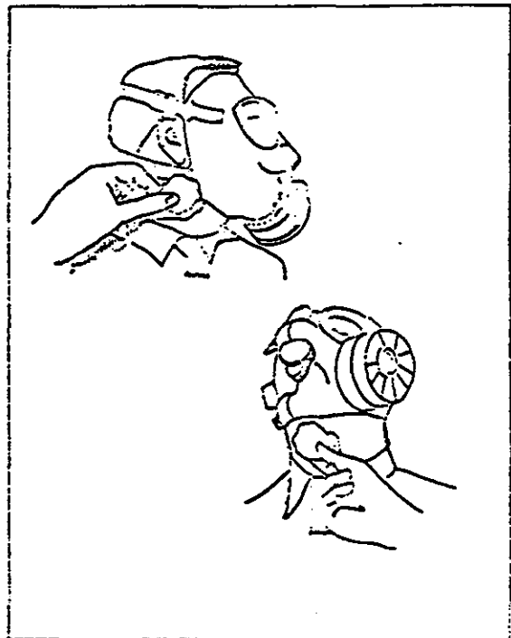
Fig. 13.1. Field test of face fit of respirators using isoamyl acetate.
