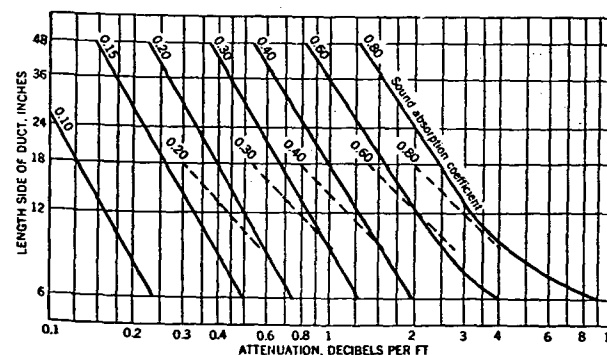
FIG. 5. SOUND ATTENUATION FOR VARIOUS ABSORBING DUCT LINERS
