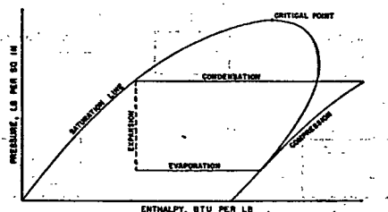
FIG. 4. PRESSURE-ENTHALPY DIAGRAM FOR SIMPLE SATURATION CYCLE
