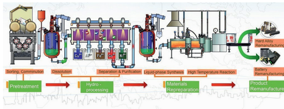
Figure 12: Flow chart of Ni/Co waste and Li-ion battery recycling process published by GEM [37]
