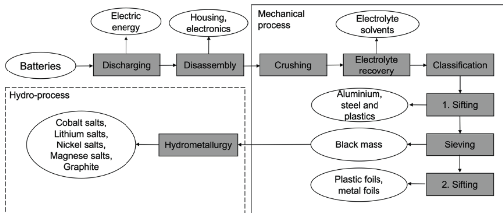
Figure 13: Mechanical recycling process published by Duesenfeld [57]
