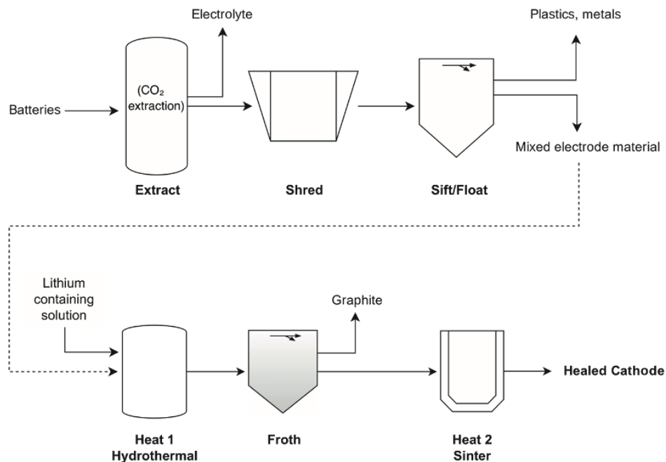
Figure 17: Direct recycling process with extraction of electrolyte with \text{CO}_2 [81]
