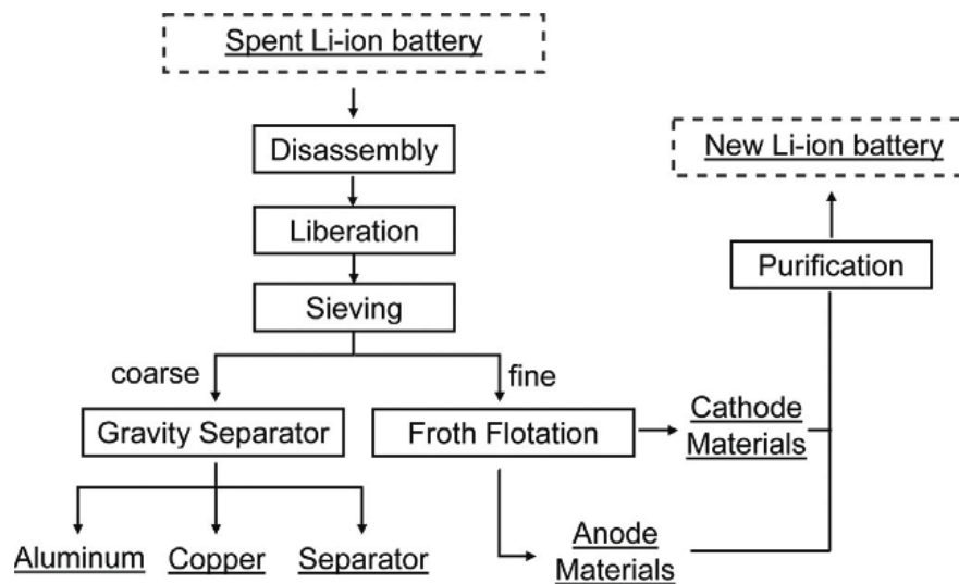
Figure 18: Recycling process with froth flotation separation of active masss [82]
