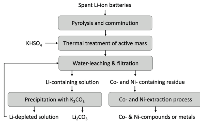
Figure 21: Flowchart of lithium extraction process with sulphate roasting (based on [86])
