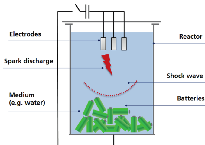
Figure 19: Electrohydraulic Fragmentation of Li-ion battery material (by Fraunhofer IWKS)
