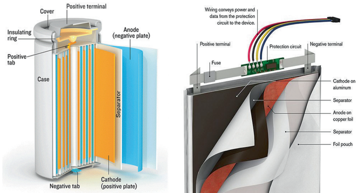
Figure 1: Constructional design of Li-ion cells (left: cylindrical, right: pouch) [2][3].
