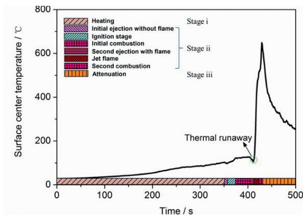
Figure 3: Example of surface temperature evolution at LIB Thermal Runaway [6]
