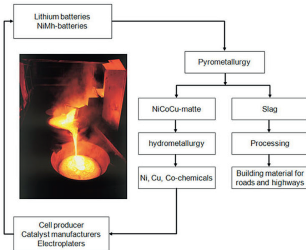
Figure 9: Li-ion&NiMH batteries recycling process published by Nickelhütte Aue [19]
