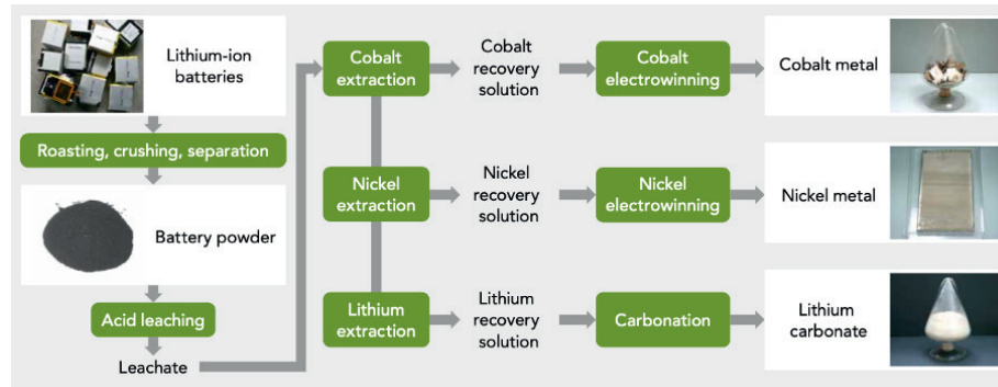
Figure 15: Flow chart of Li-ion battery recycling process published by JX Nippon Tsuruga [69]
