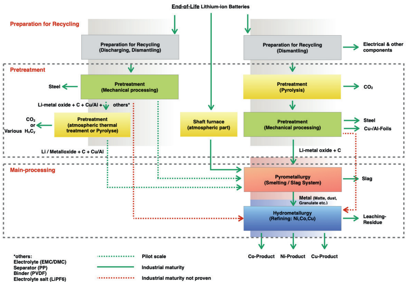
Figure 5: Overview about schematized Li-ion batteries recycling routes
