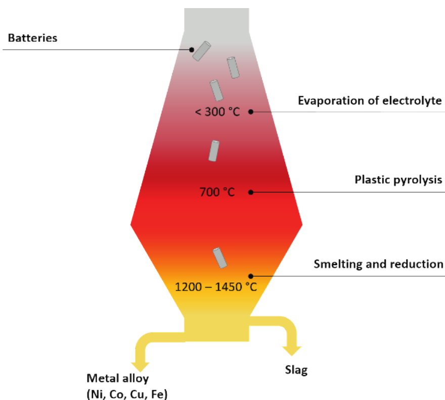
Figure 7: Schematic diagram of Umicore's shaft furnace [16]
