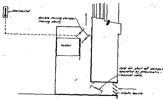
FIG. 63. DIAGRAM OF A METHOD OF CONTROL FOR A UNIT VENTILATOR
