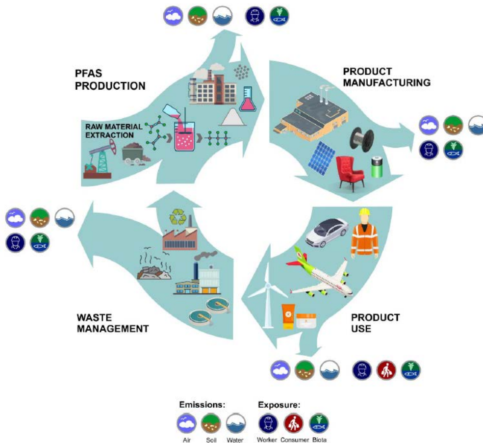
Figure 1 Emissions of and exposure to PFASs during their whole life cycle, including the waste management stage, in a circular economy.
