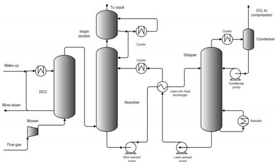
Figure 5 Process diagram of the CO 2 capture unit taken from Fernandez (2013)
