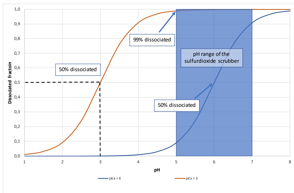
Figure 3 Fraction of the ionising substance dissociated in the SO 2 scrubber as a function of the pH and the acid dissociation constant, pKa
