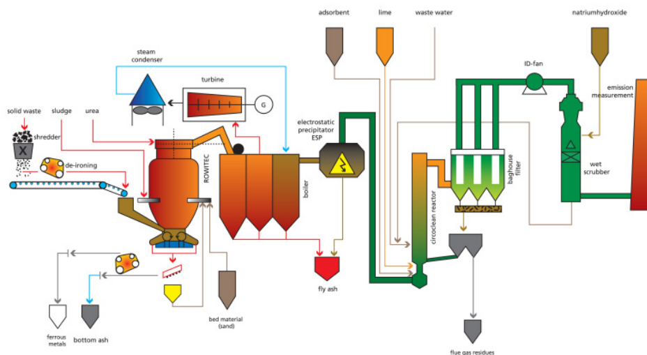
Figure 6 Schematic representation of a fluidised bed incinerator including flue gas treatment system
