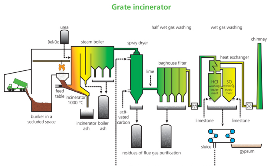
Figure 8 Schematic overview of a grate incinerator including flue gas treatment system
