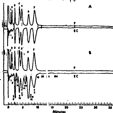
Fig. 5. Differentiation of Aroclor 1254 and organophosphorus pesticides using dual detectors and effluent split. Chromatogram A: organophosphorus standard pesticide mixture peak numbers 1 = 1.75 ng. of phorate, 2 = 2.0 ng. of diazinon, 3 = 5.0 ng. of Ronnel, 4 = 13.0 ng. of malathion, 5 = 5.0 ng. of parathion, 6 = 15.0 ng. of methyl Trithion, and 7 = 10.0 ng. of ethion. Chromatogram B: combination of organophosphorus mixture (chromatogram A) and 10 ng. of Aroclor 1254 numbered 1 to XIV as in chromatogram B of Figure 1 (a compromise of the E.C. response is necessary to obtain maximum response on the phosphorus detector). P = phosphorus detector and EC = electron capture detector. Column four percent OV-100/six percent OV-810 on 60/60 mesh Chromosorb W (AW); other GLC parameters as in Figure 1.
