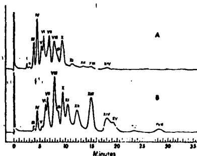
Fig. 3. Comparison of Aroclors 1254 and 1260. Chromatogram A: 5 \mu g. of Aroclor 1254; the 14 major peaks are numbered I to XIV as in chromatogram B of Figure 1. Chromatogram B: 5 \mu g. of Aroclor 1260; the 17 major peaks are numbered I to XVII (the early peaks correspond to those in Aroclor 1254). GLC parameters as in Figure 1.
