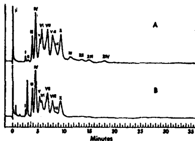
Fig. 7. Resin powder extract indicating the presence of PCB's of the Aroclor 1254 type. Chromatogram A: 5 mg. of Aroclor 1254 numbered I to XIV as in chromatogram B of Figure 1. Chromatogram B: The equivalent of 0.02 mg. of resin powder extract (hexane portion of Florisil split), numbered I to XIV as in Aroclor 1254. GLC parameters as in Figure 1
