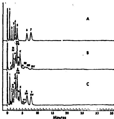
Fig. 2. Separation of PCB's and organochlorine pesticides on polar phase column (five percent DEGS/two percent H 2 PO 4 ). Chromatogram A: standard mixture of organochlorine pesticides with same amounts as in Figure 1; peak numbers: 1 = heptachlor and aldrin, 2 = lindane, 3 = heptachlor epoxide, 4 = DDE, 5 = dieldrin, 6 = DDT, 7 = DDD. Chromatogram B: 5 ng. of Aroclor 1254 (the 14 major peaks are numbered I to XIV as in chromatogram B of Figure 1, assuming that the order of elution is unchanged). Chromatogram C: combination of organochlorine standard pesticide mixture and Aroclor 1254. Other GLC parameters as in Figure 1.
