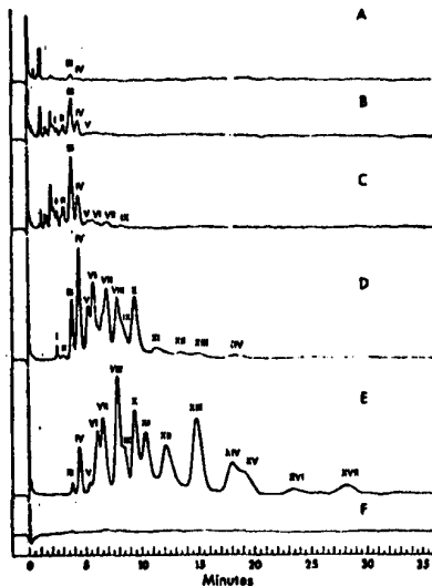
Fig. 4. CLC profiles of the more popular Aroclor mixtures under normal analytical conditions. Note: All peak numbers correspond to those of Aroclor 1254. Chromatograms: A = 5 ng. of Aroclor 1221, B = 5 ng. of Aroclor 1232, C = 5 ng. of Aroclor 1242, D = 5 ng. of Aroclor 1254, E = 5 ng. of Aroclor 1260, and F = 5 ng. of Aroclor 5460. CLC parameters as in Figure 1
