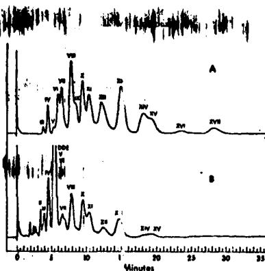
Fig. 6. Typical sample indicating the presence of PCB's of the Aroclor 1260 type in a duckling from the Toronto area. Chromatogram A: 5 mg. of Aroclor 1260 numbered I to XVII as in chromatogram B of Figure 3. Chromatogram B: the equivalent of 0.35 mg. of duck sample (hexane portion of Florisil split). Note the DDE contribution to PCB peak V. GLC parameters as in Figure 1
